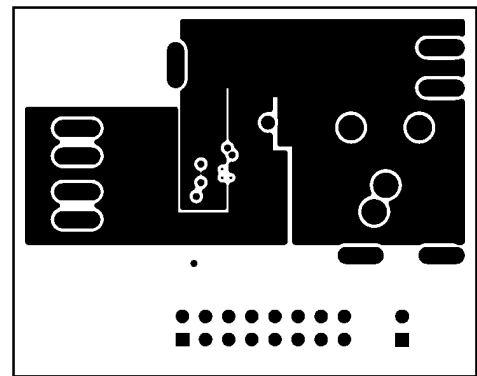
FIGURE 12. Layer 2 (GND)
