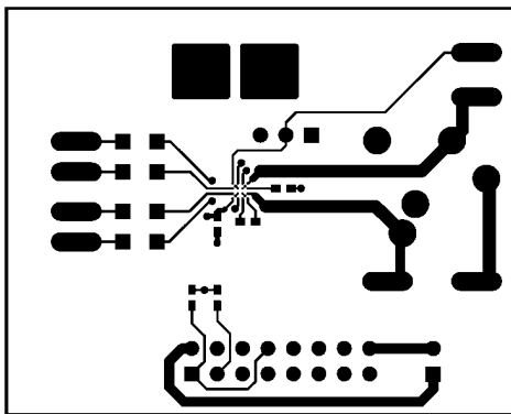
FIGURE 11. Top Layer
