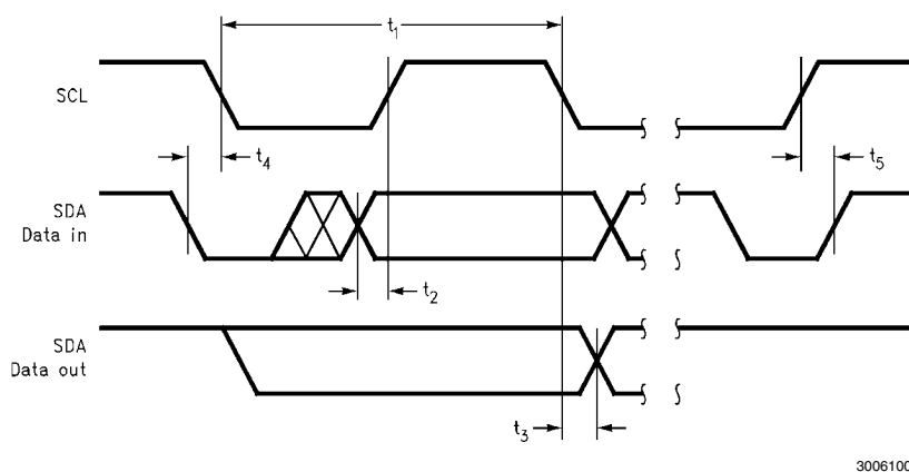
FIGURE 2. I 2 C Timing Diagram
