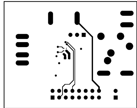
FIGURE 14. Bottom Layer
