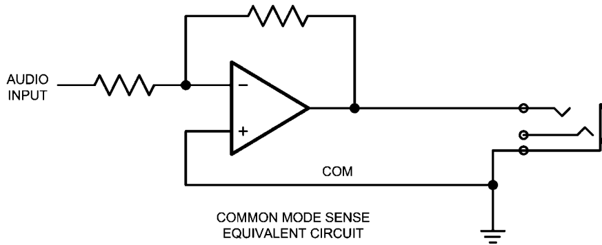
FIGURE 6. COM Connection Example
