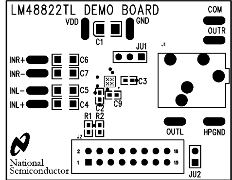
FIGURE 10. Top Silkscreen
