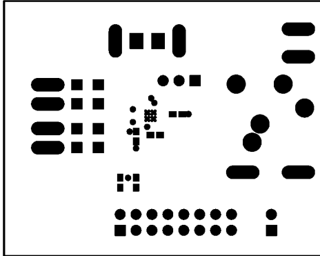
FIGURE 9. Solder Mask
