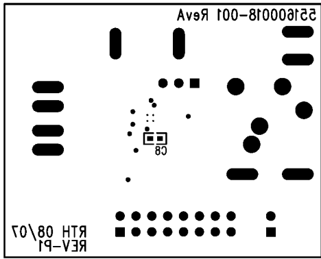
30061060 FIGURE 15. Bottom Silkscreen
