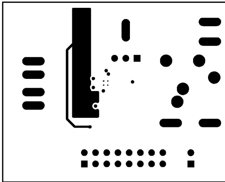
FIGURE 13. Layer 3 ( V_{DD} )
